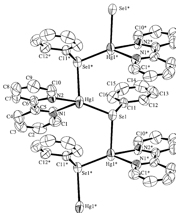
Fig. 2 Perspective drawing of three units of the complex cation of [\text{Hg}(\mu\text{-SeC}_6\text{H}_5)(\text{bpy})]_n[\text{PF}_6]_n 5 . The coordinates of the Se atom at the top are x, 1 + y, z and of the Hg(1) atom at the bottom are x, -1 + y, z . Other details as in Fig. 1.
