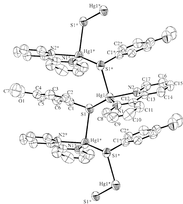
Fig. 1 Perspective drawing of three units of the complex cation of [\text{Hg}(\mu\text{-SC}_6\text{H}_4\text{OCH}_3\text{-}p)(\text{bpy})]_n[\text{PF}_6]_n 3 with the atomic numbering scheme. Hydrogen atoms have been omitted for clarity. Thermal ellipsoids are shown at the 40% probability level. The coordinates of the S atom at the top are x, 1 + y, z and of the Hg(1) atom at the bottom are x, -1 + y, z .
